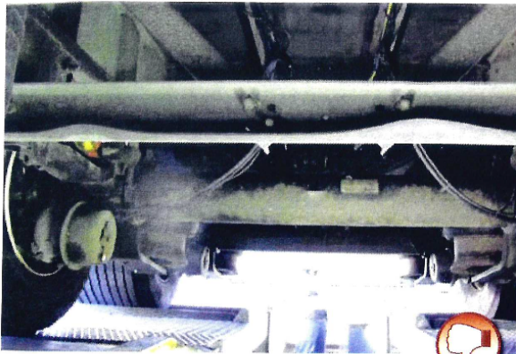
Frame cross-piece Bent frame cross-piece through wrongly positioned vehicle jack
